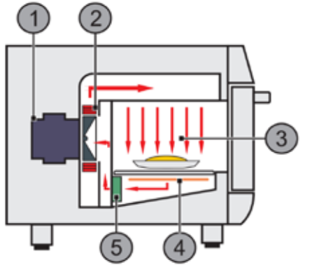
Rocket Express Teknik İllüstrasyonu Technical Illustration of Rocket Express
