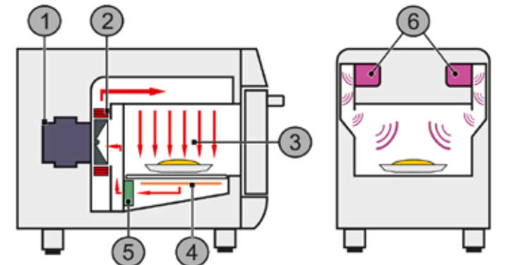
Chef Express Teknik İllüstrasyonu Technical Illustration of Chef Express
